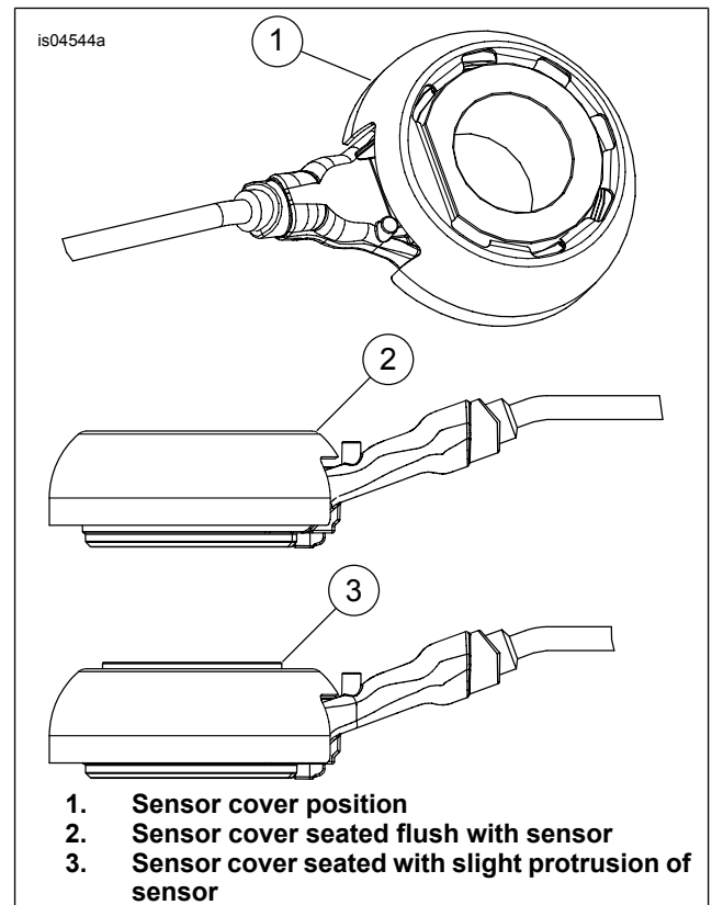
Figure 1. ABS Sensor Cover
