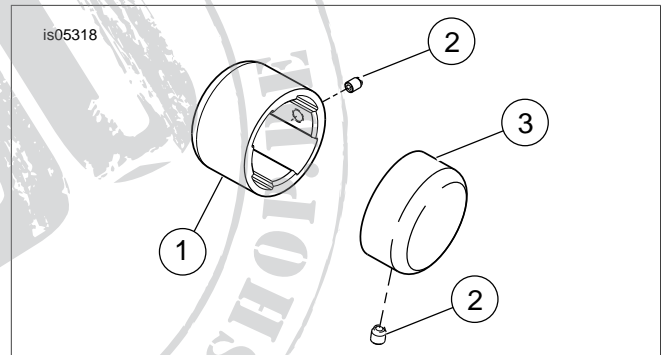
Figure 1. Service Parts: Rear Axle-Nut Cover Kit
