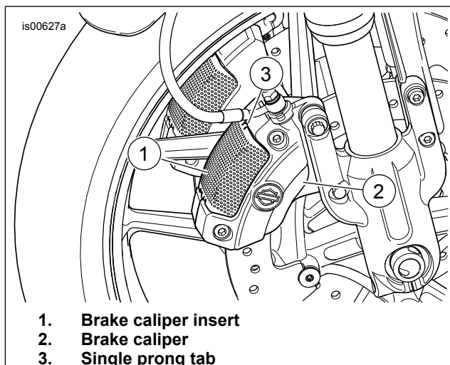
Figure 1. Front Brake Caliper (VRSCR Model Shown)
