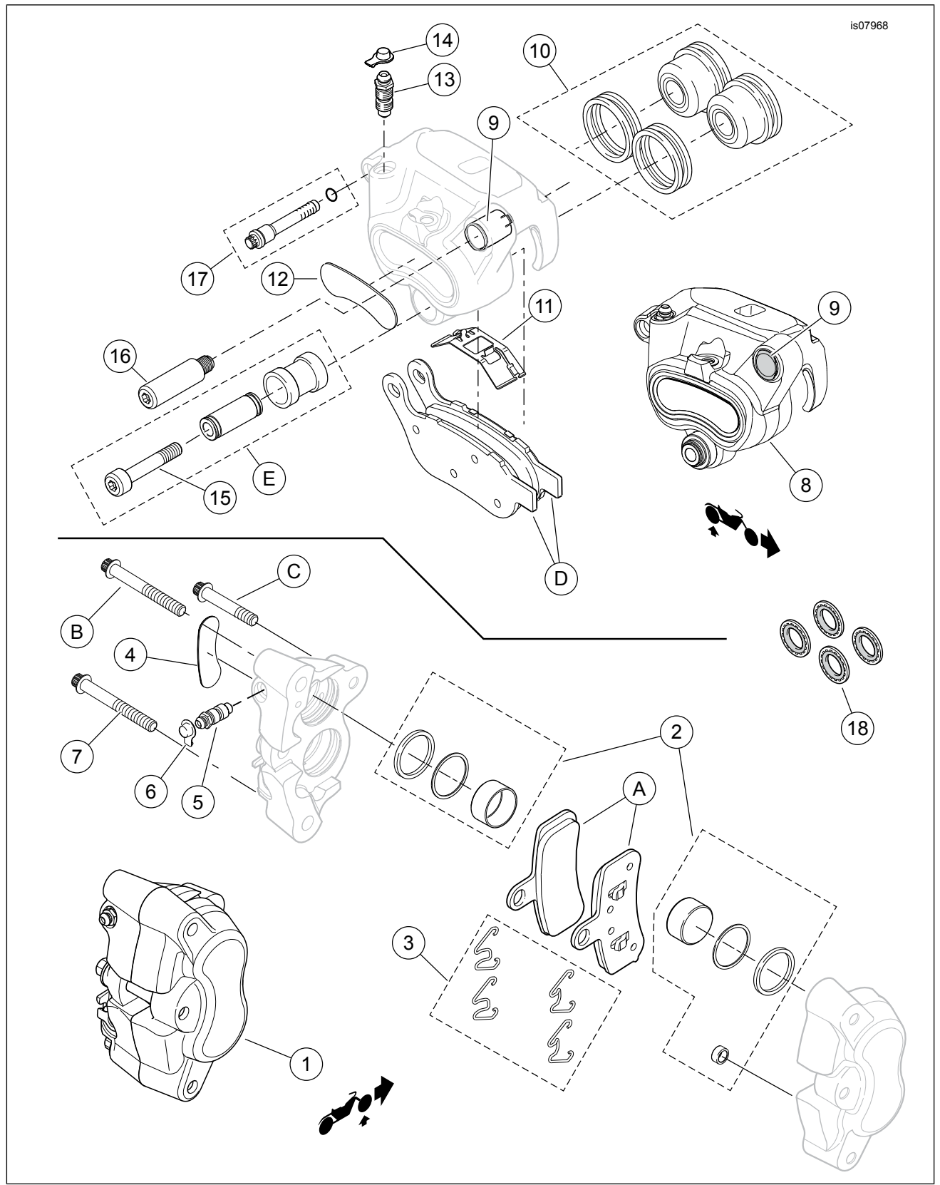
Figure 1. Service Parts, Brake Caliper Kit
