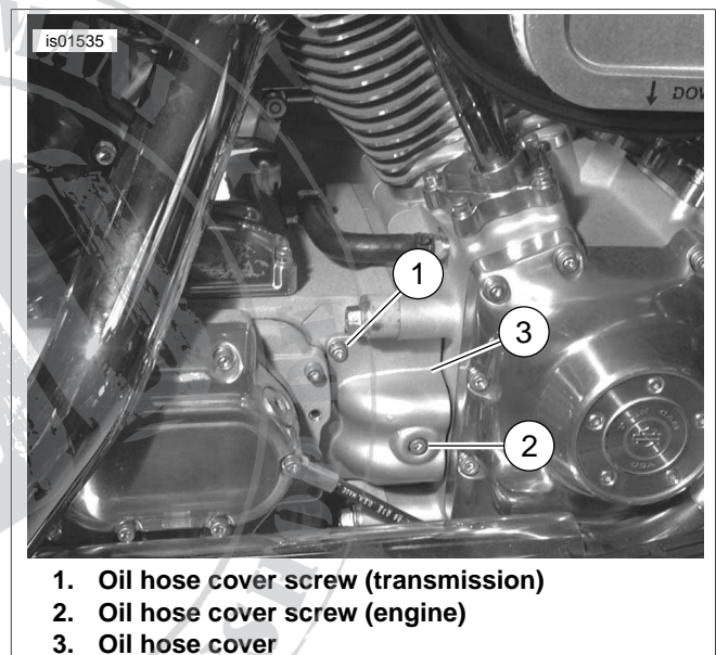
Figure 1. Oil Hose Cover Screws
