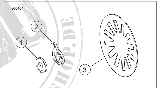
Figure 1. Service Parts for Reduced Effort Clutch Kit
