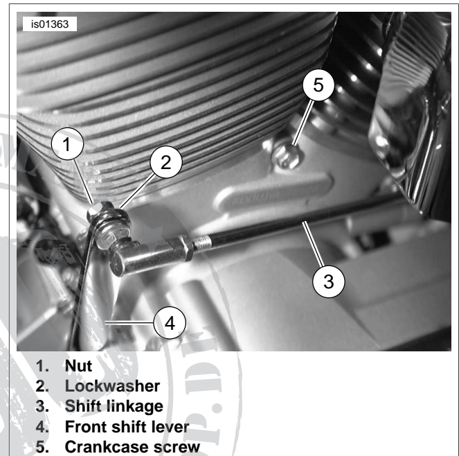
Figure 1. Remove Front of Shift Linkage and Center
