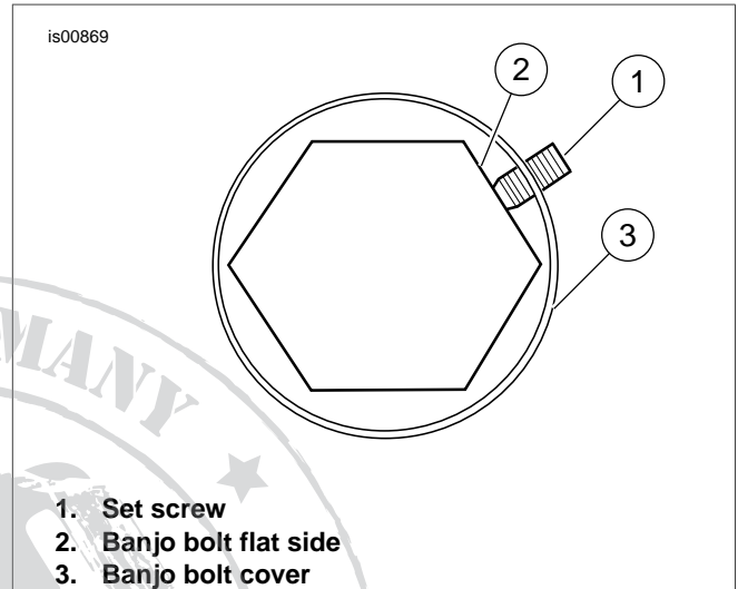
Figure 2. Set Screw Orientation
