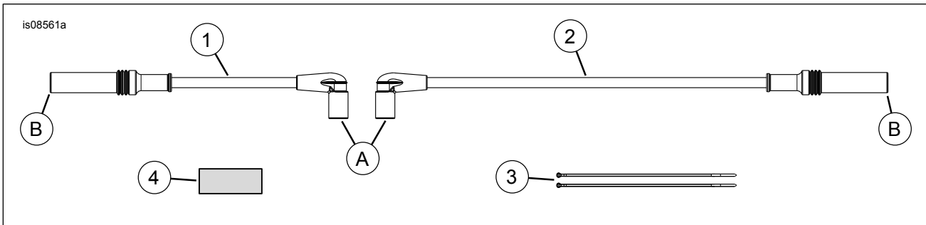
Figure 3. Service Parts: Screamin Eagle 10 MM Spark Plug Cables
