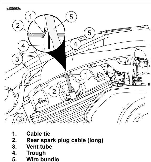
Figure 2. Secure Spark Plug Cable (shown without fuel tank and seat for clarity)
