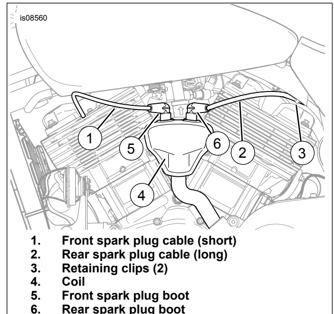
Figure 1. Spark Plug Cables
