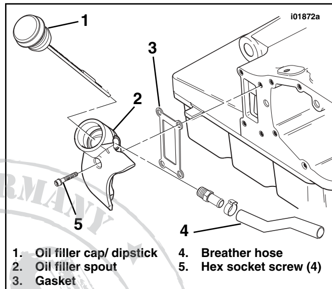
Figure 1. Remove Oil Filler Spout (FLT Models Only)
