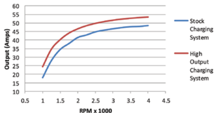
Stock Big Twin vs. High Output Charging System
