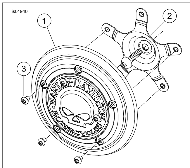
Figure 1. Service Parts: "Skull" Air Cleaner Cover
