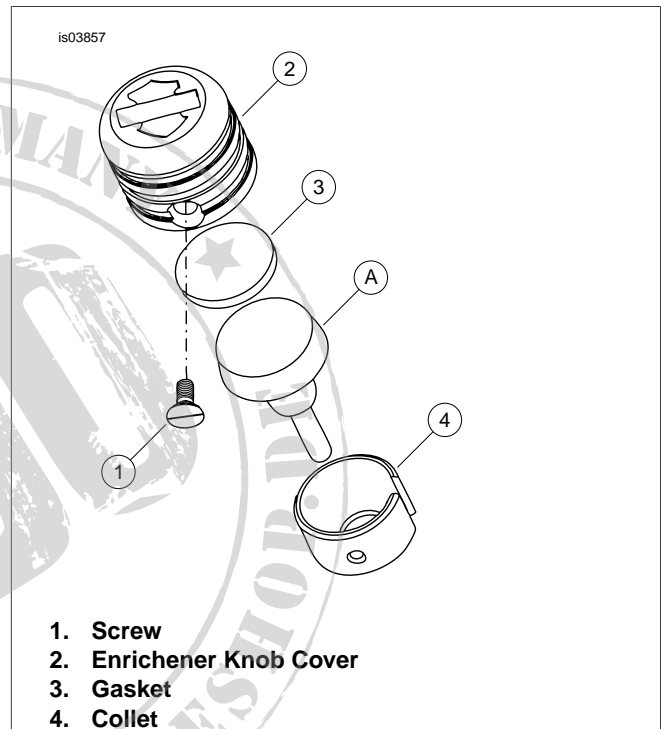
Figure 1. Enrichener Knob Cover Installation
