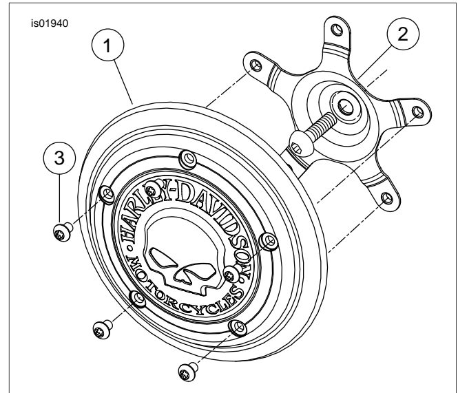
Figure 1. Service Parts: "Skull" Air Cleaner Cover
