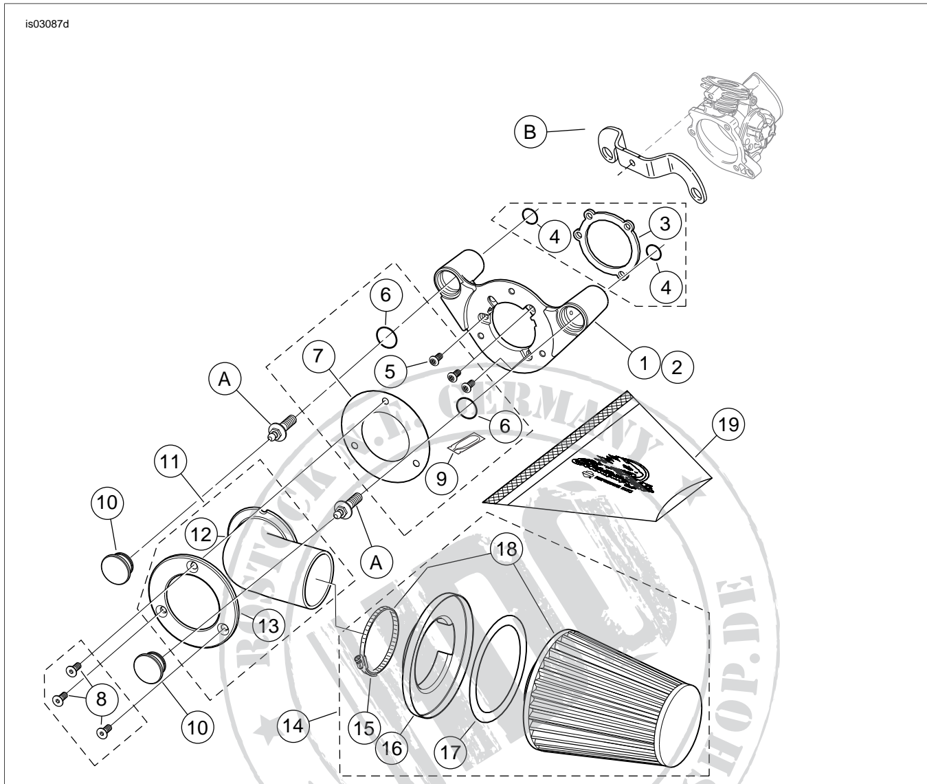
Figure 1. Service Parts: Air Cleaner Kit
