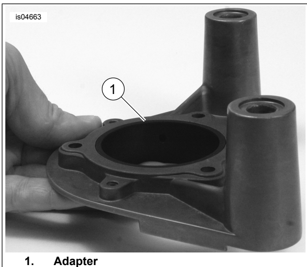
Figure 2. Adapter Positioned Correctly in Backplate
