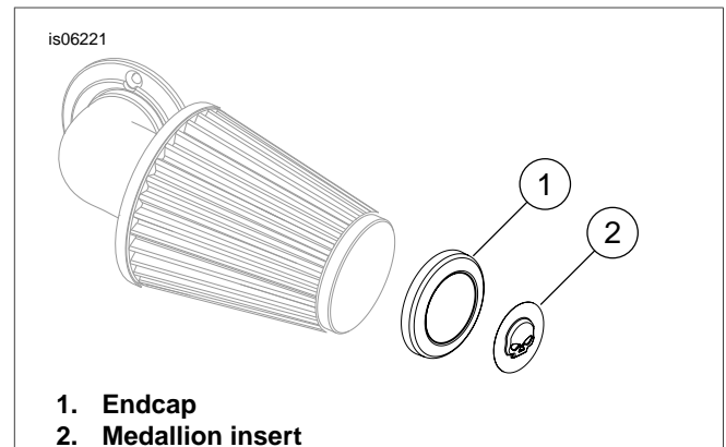
Figure 1. Install Endcap to Air Cleaner
