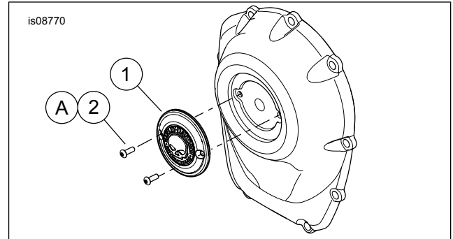
Figure 1. Timer Cover Kits: 25600064, 25600065, 25600066, 25600067, 25600068
