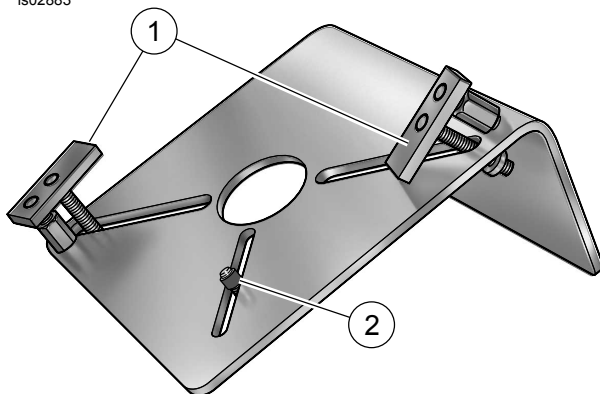
Figure 2. Flywheel Fixture (Part Number HD-44358)
