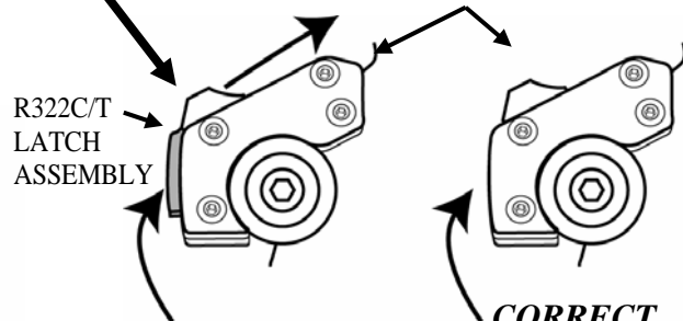
2320-0065 FATS/SLIMS PLATE ONLY MOUNTING KIT
