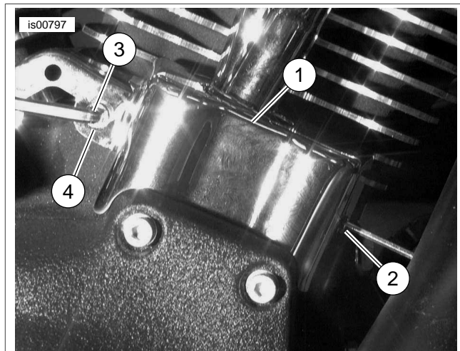
Figure 3. Center Lifter Cover Bracket Installation
