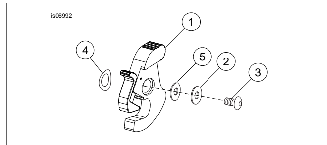
Figure 2. Service Parts: Rotary Latch Kit
