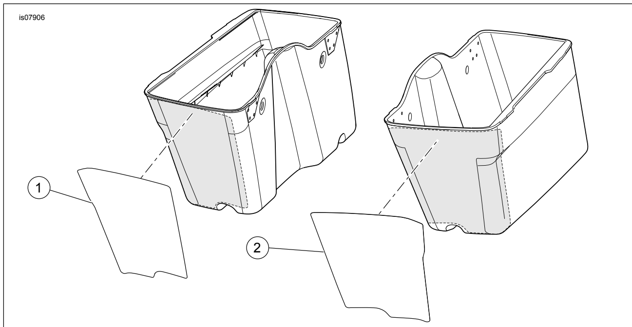
Figure 1. Service Parts: Paint Guard Kit
